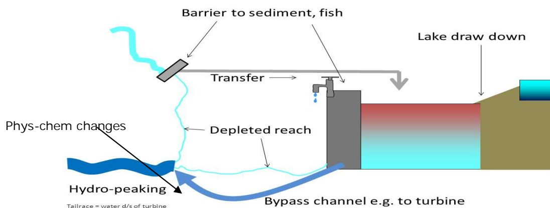
Figure 1. Typical hydromorphological alterations giving ecological impacts to water bodies from water storage (for hydropower, drinking-water supply, irrigation or other equally important sustainable activities as stated in Article 4.3 of WFD).
