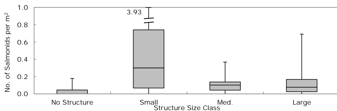
Figure 11. Number of salmonids observed per square meter of habitat in engineered logjams of different sizes and nearby control areas without structures.
