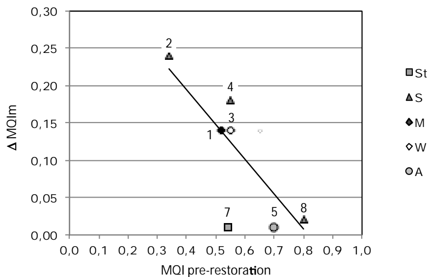
Figure 2. Increment of MQIm ( \Delta MQIm ) vs. initial morphological quality (MQI pre-restoration) for different channel morphologies. 1: Aurino; 2: Becva; 3: Drau; 4: Lippe; 5: Narew; 6: Thur; 7: Töss; 8: Vääräjoki.
