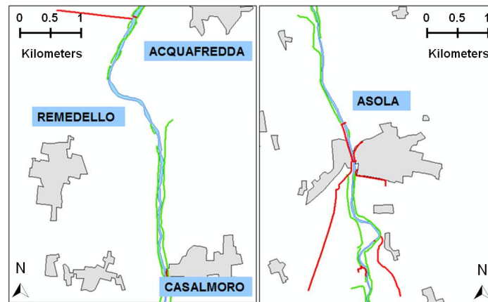
Figure 1. Two reaches of the Chiese River in the ALT_Base* (left: reach downstream of Acquafredda town; right: following downstream reach). The green lines indicate currently existing works that would be dismissed in such an alternative, while the red ones indicate works (existing or planned by SdF or newly proposed by us) which would be kept in ALT_Base*.
