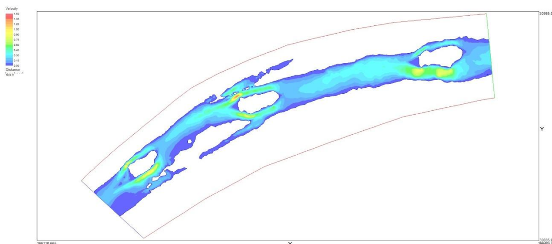
Figure 1. Velocity flow fields simulated with the River2D for the selected scenario of islands in the mid-section of the channel.
