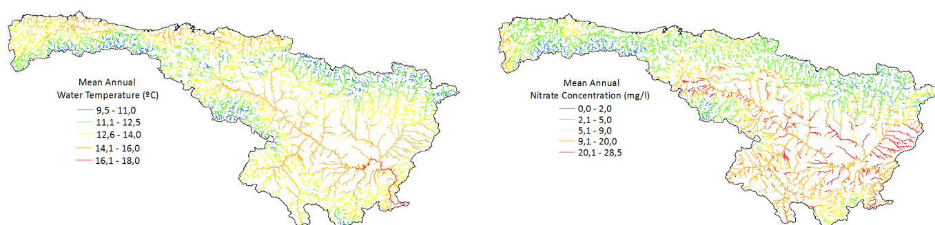
Figure 4. Mean annual water temperature and nitrate concentration obtained using Random Forest models in which more than 250 water quality sites were used in the northern fourth of the Iberian Peninsula (Álvarez-Cabria et al. , In Press).
