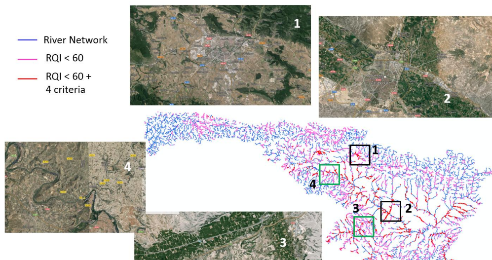
Figure 5. Spatial results after querying a SRN-GIS database for river reaches with bad conservation status for riparian vegetation (RQI <60: almost 4500 km a 14% of the total river network length), and having a high annual water temperature (> 15°C), high nitrate concentration (>10 mg/l), high bank cliff abundance and high potential for floodplain restoration (> 250 m). These river reaches supposed a 15% (690 km) of the sites with bad riparian vegetation conservation status.
