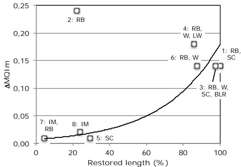
Figure 3. Increment of MQIm ( \Delta MQIm ) vs. restored length. 1: Aurino; 2: Becva; 3: Drau; 4: Lippe; 5: Narew; 6: Thur; 7: Töss; 8: Vääräjoki. Restoration measures: RB: removal of bank protections and/or artificial levées; W: channel widening; SC: reconnection or construction of secondary channels; BLR: bed level raising; IM: instream measures for habitat enhancement; LW: introduction of large wood.
