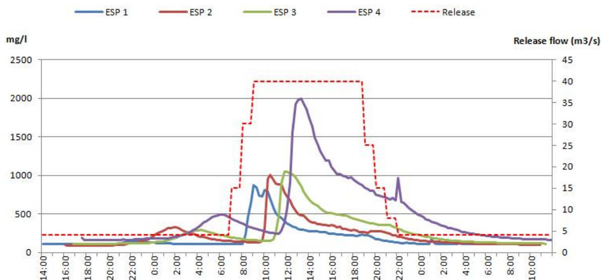
Figure 2. Release flow and TSS at each station (Espinasses, Nov. 14, 2014).
